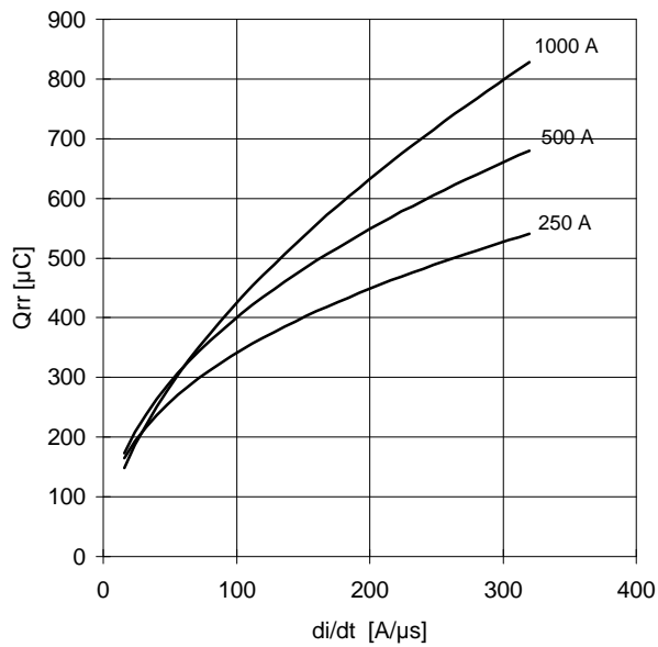
REVERSE RECOVERY CHARGE Tj = 150 °C
